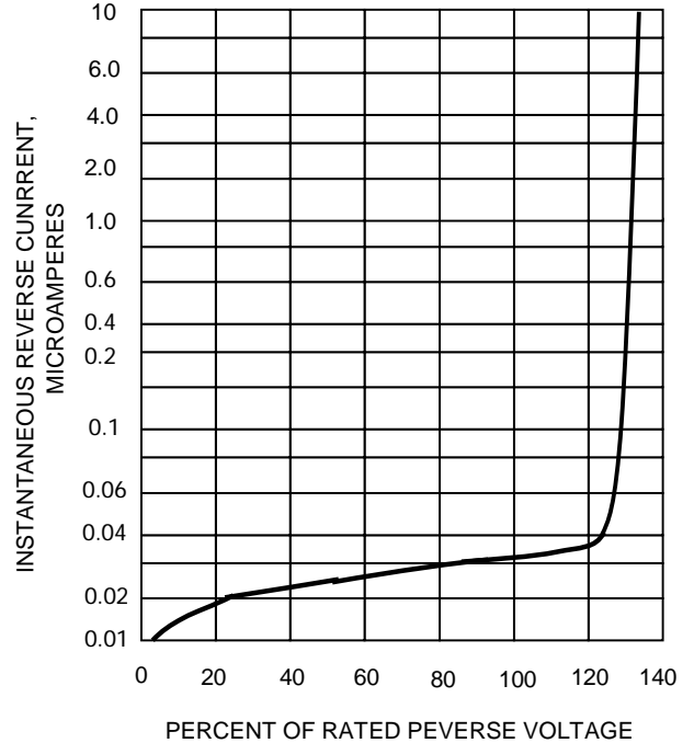
FIG.4-TYPICAL REVERSE CHARACTERISTICS
